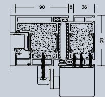
Snit H-H
