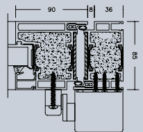
Snit F-F
